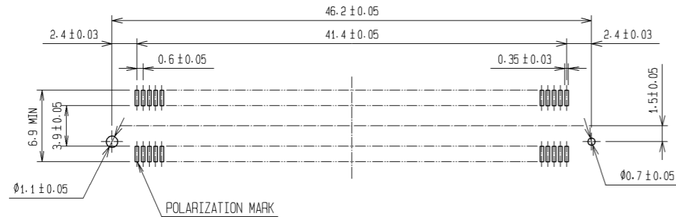
RECOMMENDED LAND PATTERN DIMENSION OF PCB (MOUNTING SIDE) (2:1) (RECOMMENDED METAL MASK THICKNESS:0.15mm)
