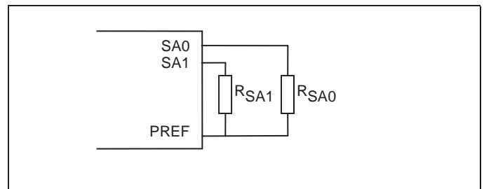
Schematic of connection of address resistor.
